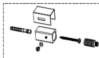
bracket accessory 2:1
