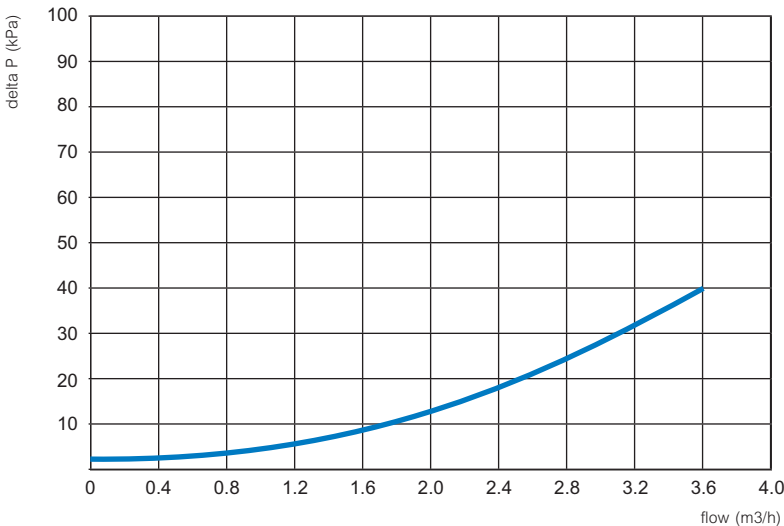
Pressure loss-curve
