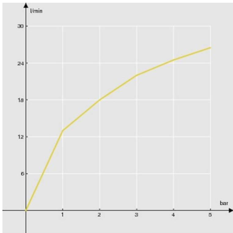
FLOW RATE DIAGRAM: Mixed Vand
